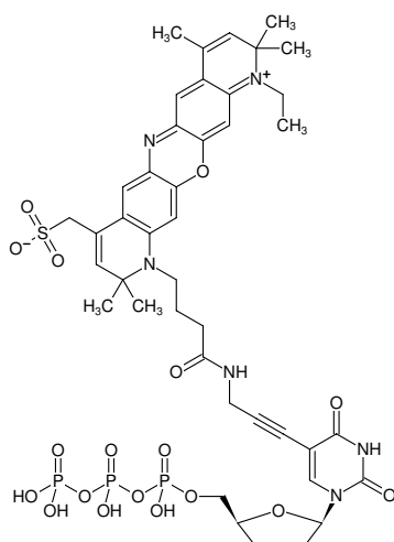
Structural formula of 5-Propargylamino-ddUTP-ATTO-700
