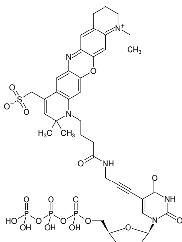
Structural formula of 5-Propargylamino-ddUTP-ATTO-680
