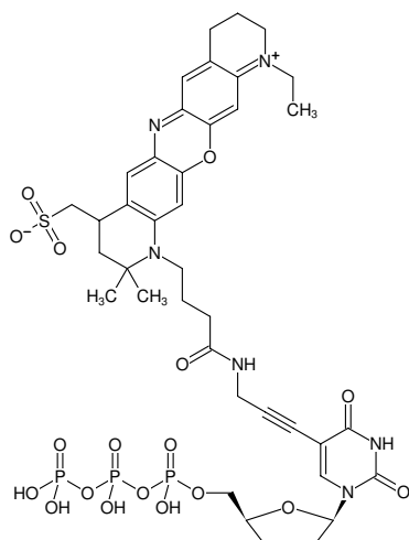
Structural formula of 5-Propargylamino-ddUTP-ATTO-655
