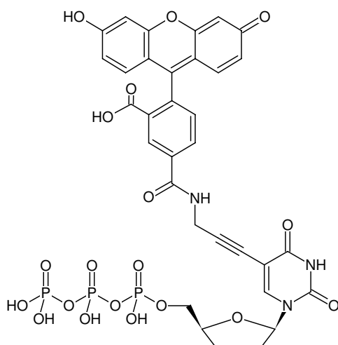
Structural formula of 5-Propargylamino-ddUTP-5-FAM
