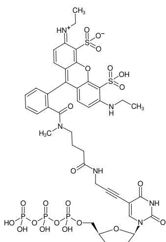
Structural formula of 5-Propargylamino-ddUTP-ATTO-532
