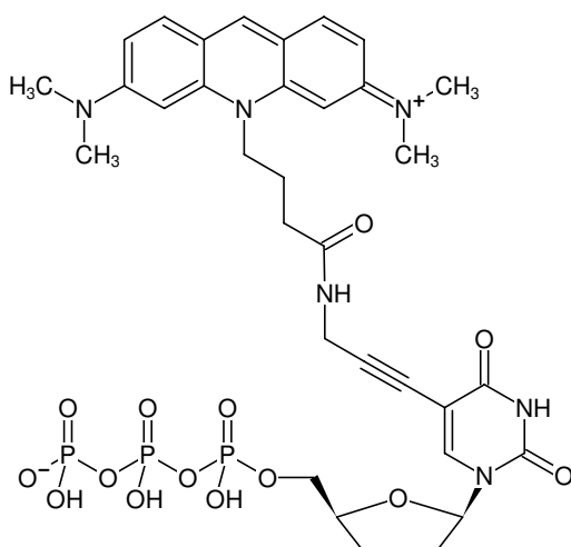
Structural formula of 5-Propargylamino-ddUTP-ATTO-495
