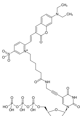
Structural formula of 5-Propargylamino-ddUTP-DY-480XL
