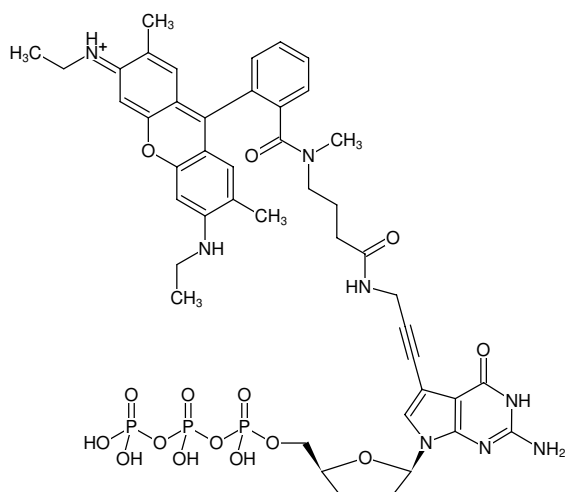
Structural formula of 7-Propargylamino-7-deaza-ddGTP-ATTO-Rho6G
