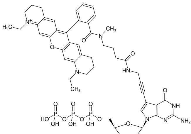
Structural formula of 7-Propargylamino-7-deaza-ddGTP-ATTO-Rho11
