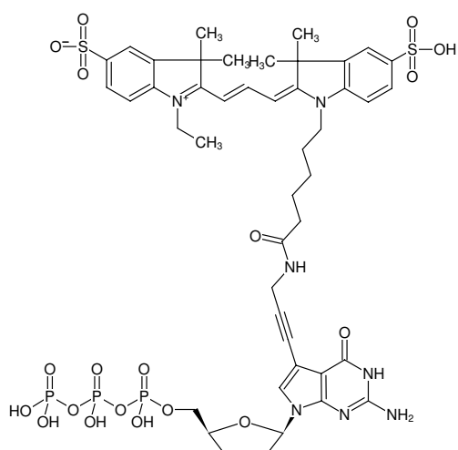
Structural formula of 7-Propargylamino-7-deaza-ddGTP-Cy3
