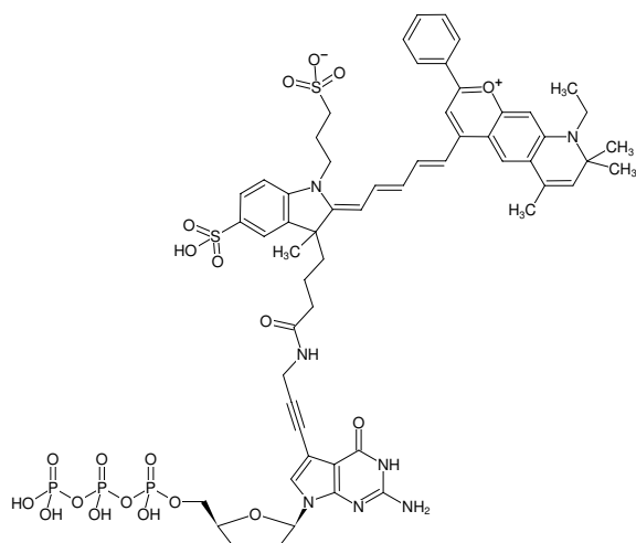
Structural formula of 7-Propargylamino-7-deaza-ddGTP-DY-776
