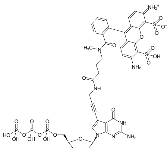
Structural formula of 7-Propargylamino-7-deaza-ddGTP-ATTO-488
