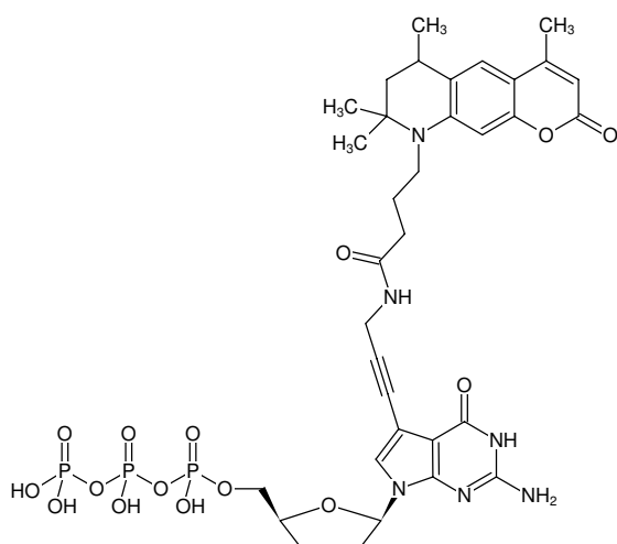
Structural formula of 7-Propargylamino-7-deaza-ddGTP-ATTO-390
