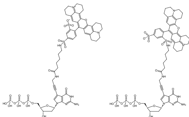
Structural formula of 7-Propargylamino-7-deaza-dGTP-Texas Red
