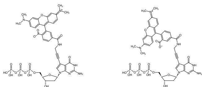
Structural formula of 7-Propargylamino-7-deaza-dGTP-5/6-TAMRA
