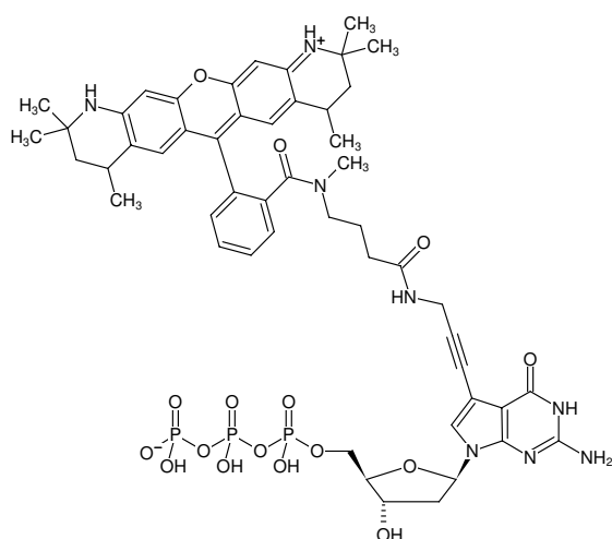
Structural formula of 7-Propargylamino-7-deaza-dGTP-ATTO-550
