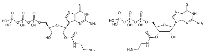
Structural formula of EDA-6-Thio-GTP
