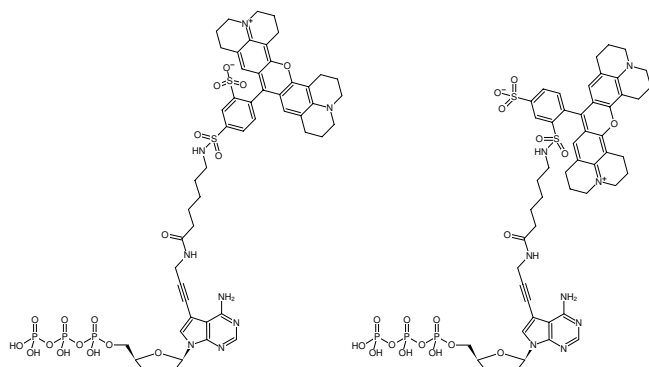
Structural formula of 7-Propargylamino-7-deaza-ddATP-Texas Red
