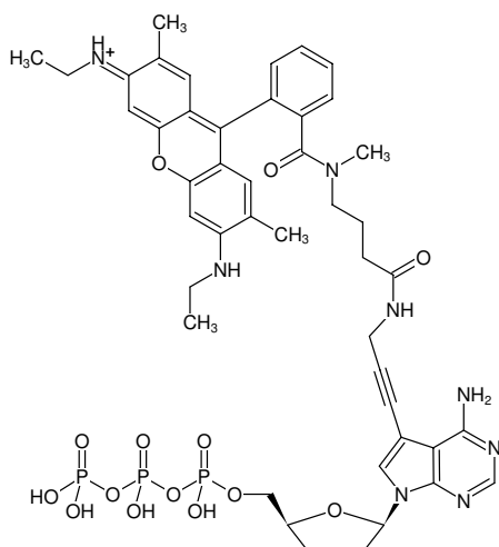
Structural formula of 7-Propargylamino-7-deaza-ddATP-ATTO-Rho6G
