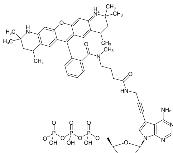
Structural formula of 7-Propargylamino-7-deaza-ddATP-ATTO-550
