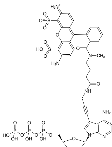
Structural formula of 7-Propargylamino-7-deaza-ddATP-ATTO-488
