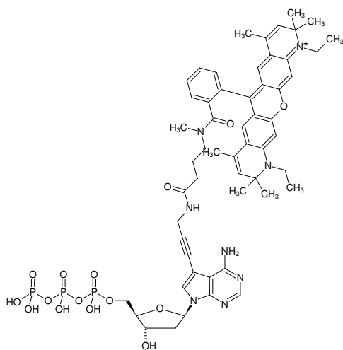
Structural formula of 7-Propargylamino-7-deaza-dATP-ATTO-Rho13
