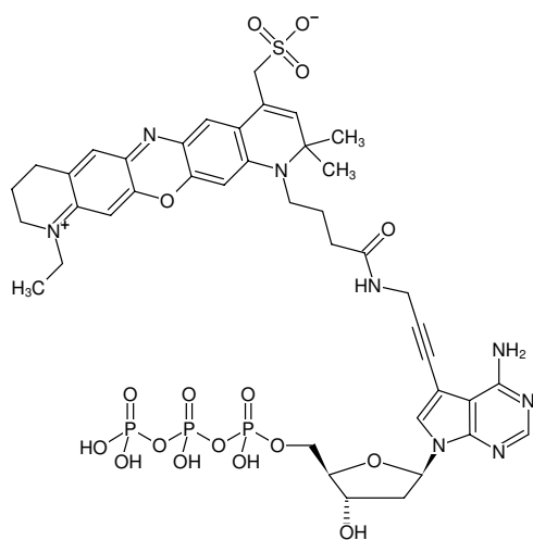
Structural formula of 7-Propargylamino-7-deaza-dATP-ATTO-680
