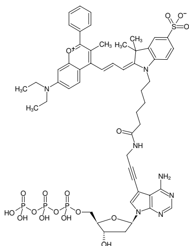
Structural formula of 7-Propargylamino-7-deaza-dATP-DYQ-660
