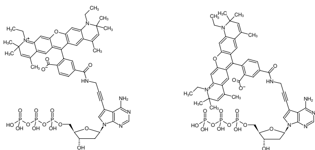
Structural formula of 7-Propargylamino-7-deaza-dATP-ATTO-590
