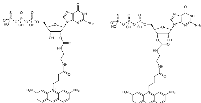
Structural formula of EDA-GTPyS-ATTO-465
