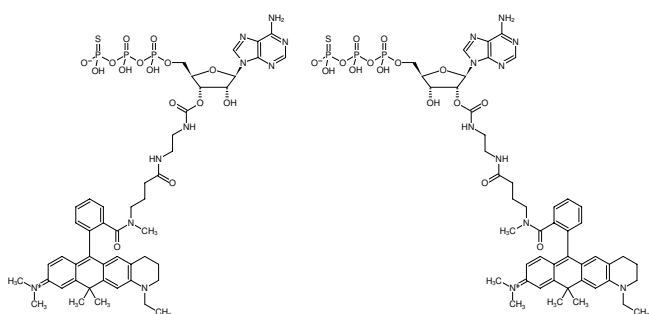
Structural formula of EDA-ATPyS-ATTO-633
