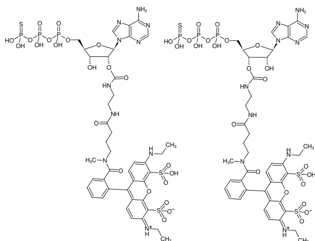
Structural formula of EDA-ATPyS-ATTO-532
