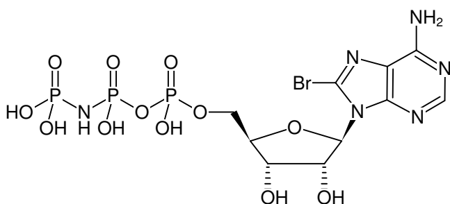
Structural formula of 8-Bromo-AppNHp
