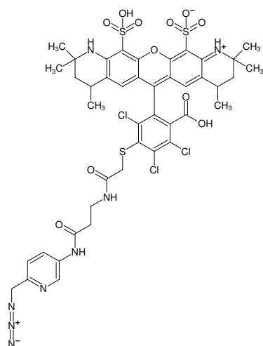
Structural formula of AF546-Picolyl-Azide
