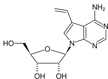
Structural formula of 7-Deaza-vinyl-adenosine (7-dVA)
