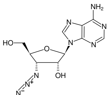
Structural formula of 3'-Azido-3'-deoxyadenosine
